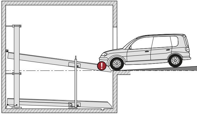
max. 10% slope
